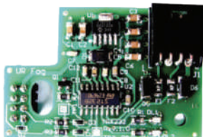
Transceiver rs232 5/12 V
